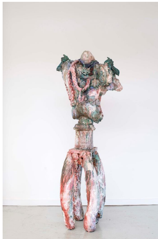
Principle of Intrusive Relationships
